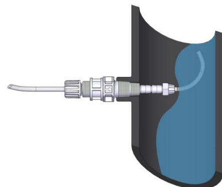
INSTALLATION ON 1/2" CONNECTION WITH ANTIFOAM 4x6 FLEXIBLE EXTENSION
